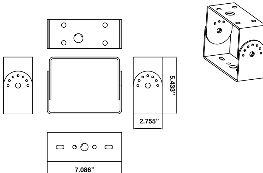
Trunnion Swivel
